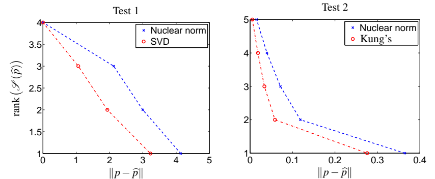
Fig. 3.1 Rank vs approximation error trade-off curve.
